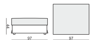
CORNER 90°
