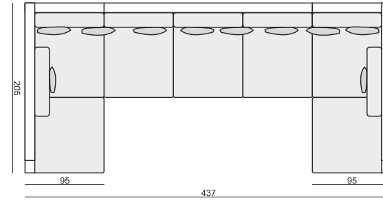
SET 2 DIVAN LEFT + 4 SEATER (two parts) without ARMRESTS + DIVAN RIGHT
