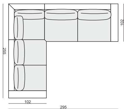
SET 8 LEFT (or RIGHT) 2 SEATER LEFT (or RIGHT) + CORNER 90° No.1 + 3 SEATER RIGHT (or LEFT)
