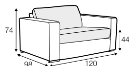
element 80
