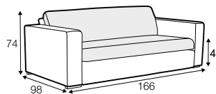
element 126
