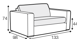
element 93
